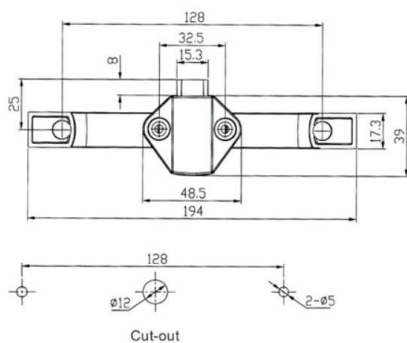
CIERRE PULSADOR MANETA PERLA ref. 152037P
