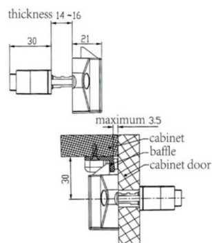
CIERRE PULSADOR MANETA NICKEL ref. 152037N
