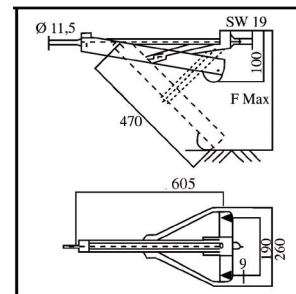
PATA RETRACTIL CHASIS ULTRALIGERO 605 MM ref. 130142
