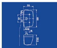
LUZ MATRICULA JOKON ref. 172410
